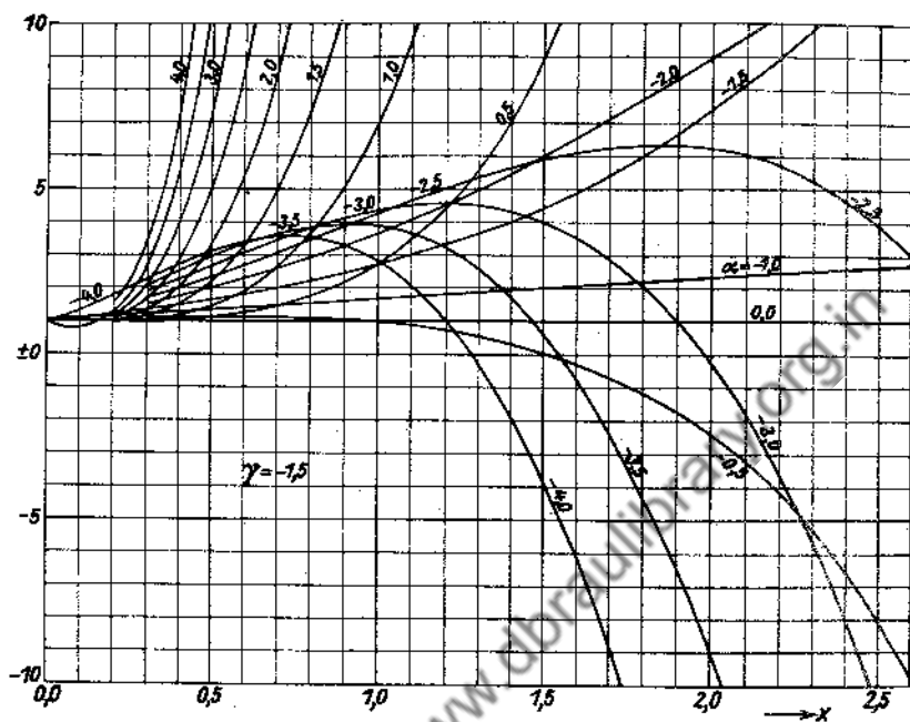
Fig. 151. M(\alpha, -1.5, x) .
