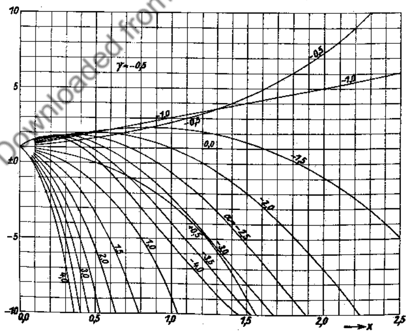
Fig. 152. M(\alpha, -0.5, x) .
