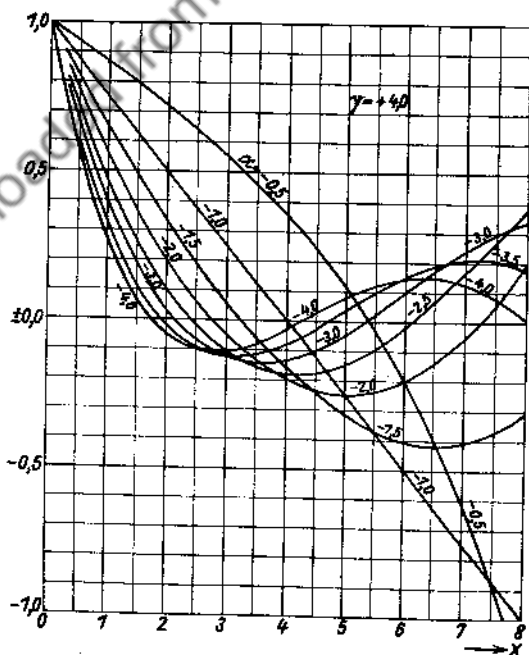
Fig. 164. M(\alpha, +4.0, x) .
