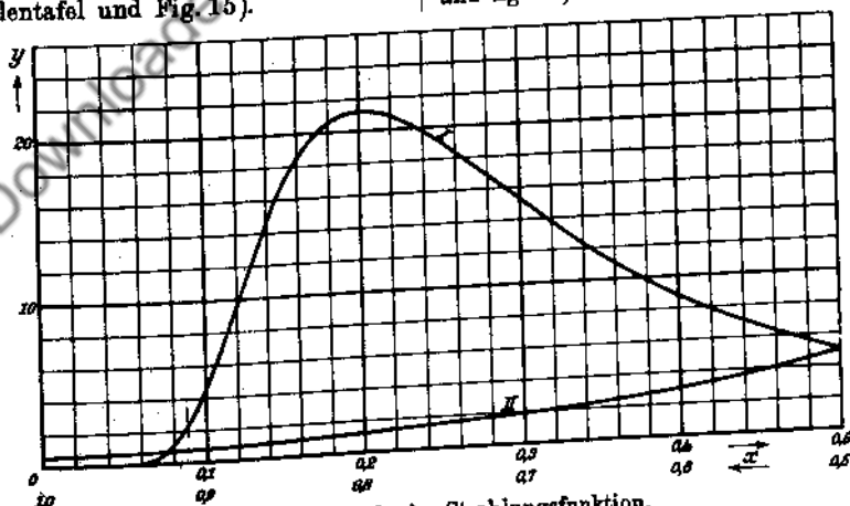
Fig. 16. Planck's radiation function.
