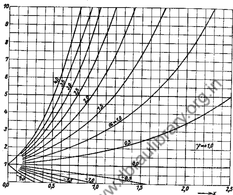
Fig. 155. M(\alpha, +1.0, x) .
