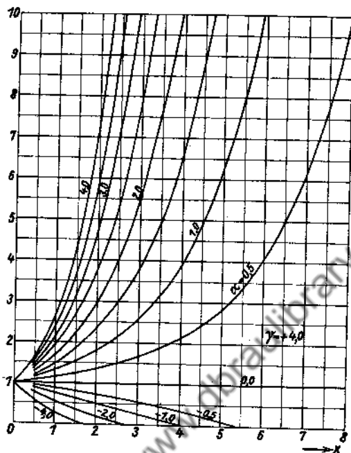
Fig. 163. M(\alpha, +4.0, x) .
