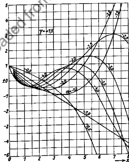
Fig. 158. M(\alpha, +1.5, x) .
