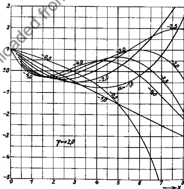
Fig. 160. M(\alpha, +2.0, x) .
