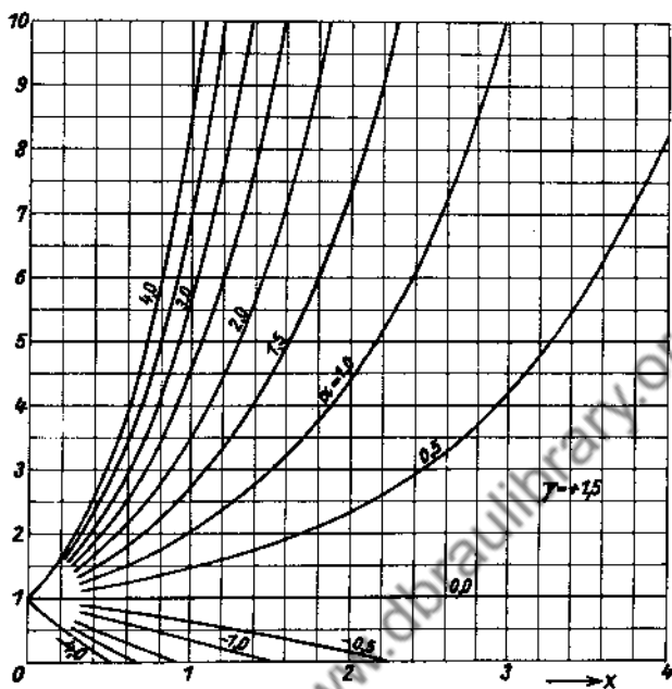
Fig. 157. M(\alpha, +1.5, x) .
