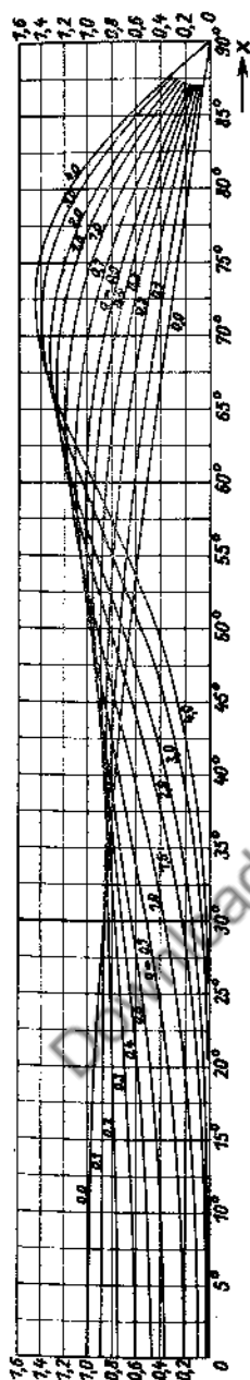
Fig. 172. ce_1(x, q) .
