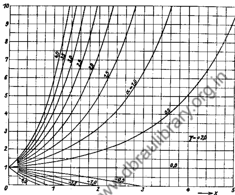
Fig. 159. M(\alpha, +2.0, x) .
