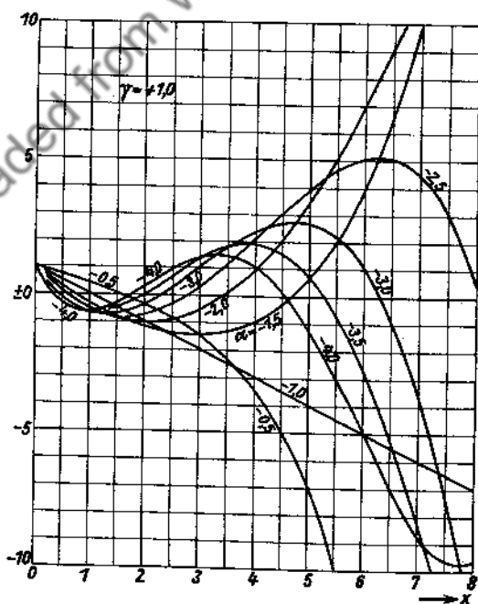
Fig. 156. M(\alpha, +1.0, x) .
