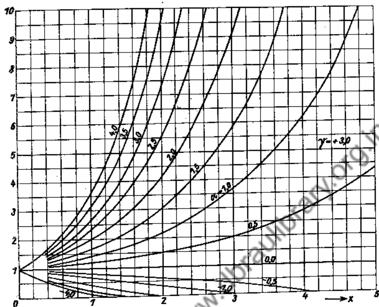
Fig. 161. M(\alpha, +3.0, x) .
