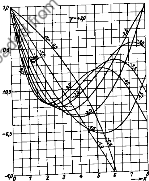
Fig. 162. M(\alpha, +3.0, x) .
